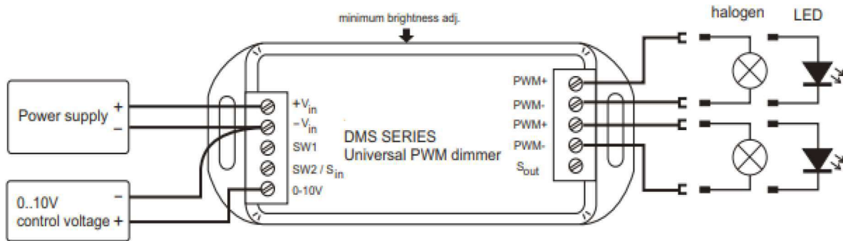
Wiring diagram for 0-10V control
